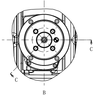
Detailed drawing of end-effector mounting face
