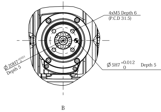
Detailed drawing of end-effector mounting face
