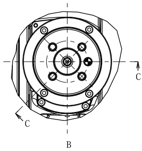
Detailed drawing of end-effector mounting face
