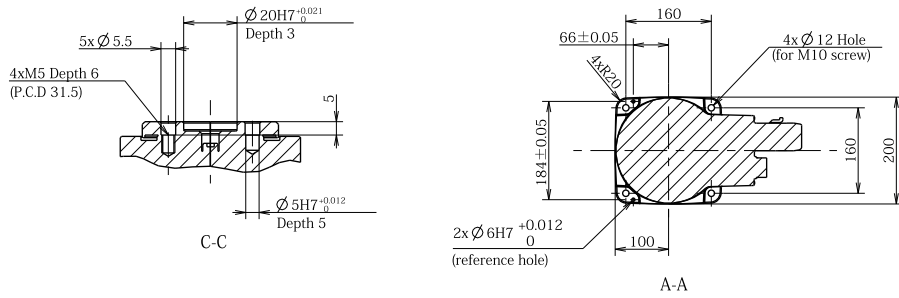
Detailed drawing of base mounting face
