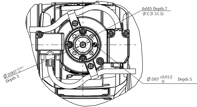
Detailed drawing of base mounting face
