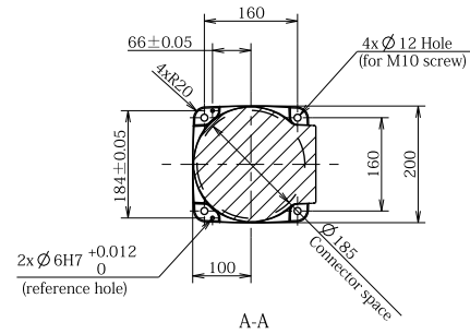
Detailed drawing of base mounting face
