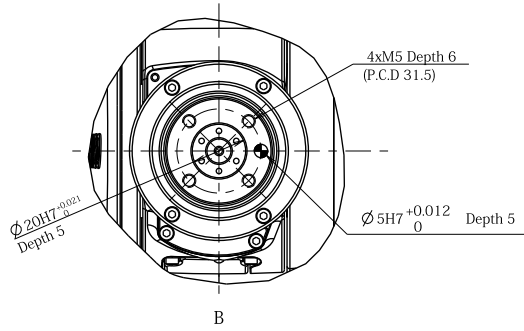
Detailed drawing of end-effector mounting face
