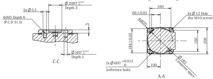
Detailed drawing of base mounting face
