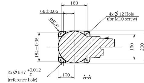
Detailed drawing of base mounting face
